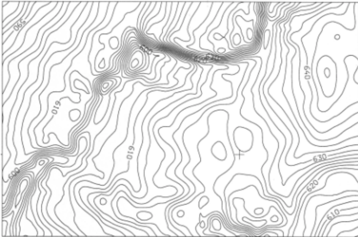
Figure 6: "Canopy surface", obtained with interpolation and filtering with a skew error distribution function on the inverse model (elevations multiplied with -1 before and back after interpolation).
