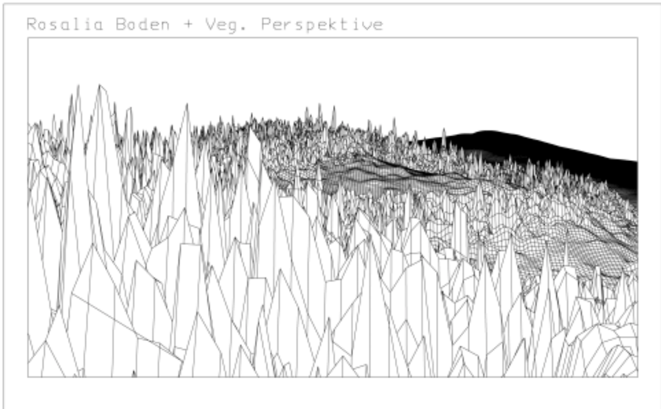
Figure 5: Perspective view of ground model with vegetation implied.
