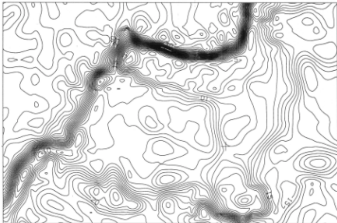
Figure 7: Difference between "canopy surface" and ground model shows stand heights.
