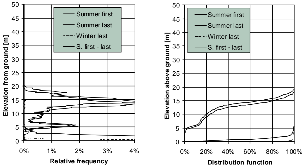
Figure 8c: Histogram and distribution function of elevation distribution of a young beech stand.
