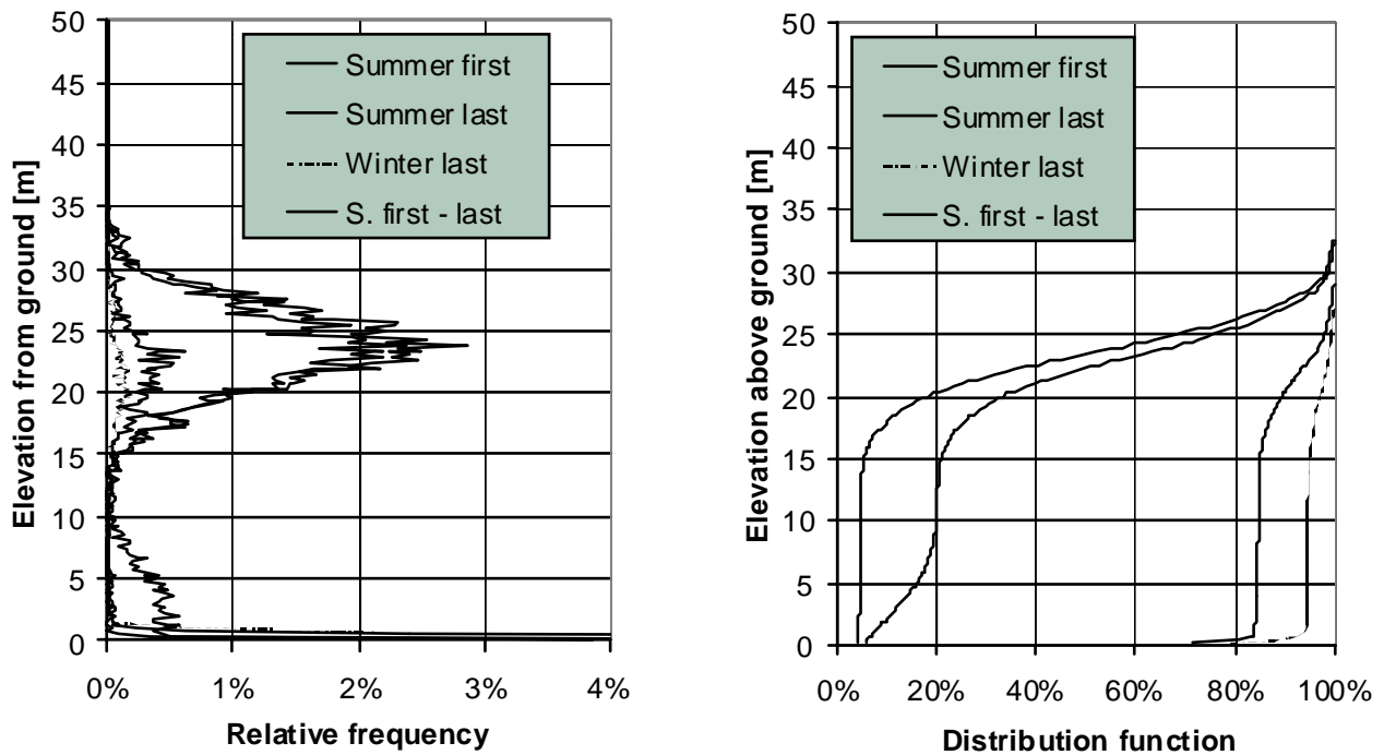
Figure 8b: Histogram and distribution function of elevation distribution of a mature spruce stand.
