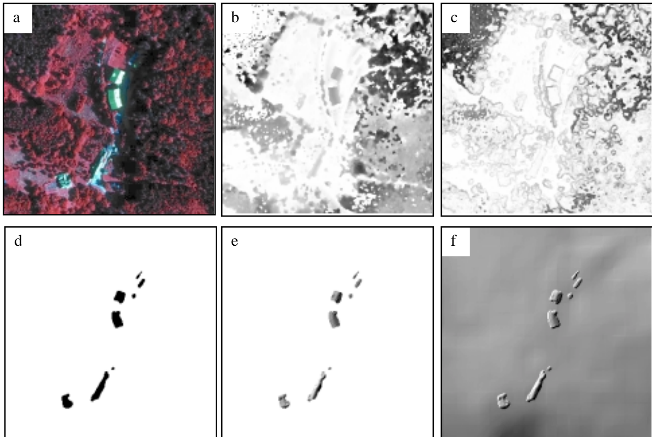
Figure 1: Separation of vegetation (trees) and solid off-terrain objects (buildings): (a) Ortho image of the area; (b) "Summer last" minus ground model, (c) "Summer first" minus "summer last"; (d) mask of buildings derived from (b) and (c) where b is higher than 1 m and c is lower than 1 m, a 3 x 3 despeckle filter was used afterwards; (e) extracted building points; (f) hill shading of DTM (ground model) with buildings implanted. Coding: Higher elevations are darker (b, c, e).
