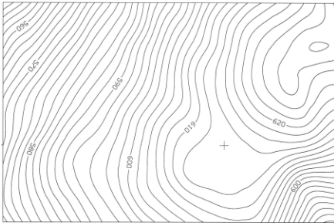
Figure 2: Terrain surface obtained from "winter last" with interpolation and filtering with a skew error distribution function.
