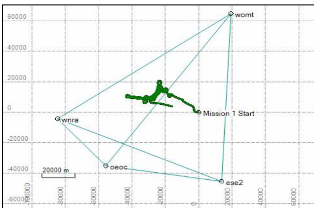
Figure 12: Reference Station Configuration
