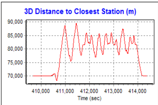
Figure 24: Distance to Nearest Station
