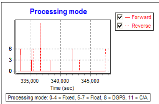
Figure 32: Processing Mode PP V5, Sharp Turns Flt2
