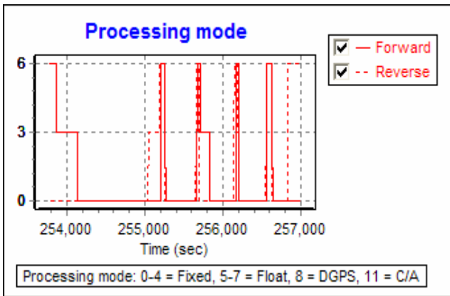
Figure 16: Processing Mode, PP V5, Partial Outages
