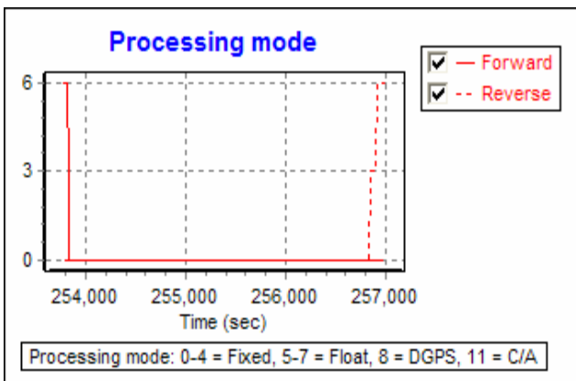
Figure 8: Solution Status, PP V5
