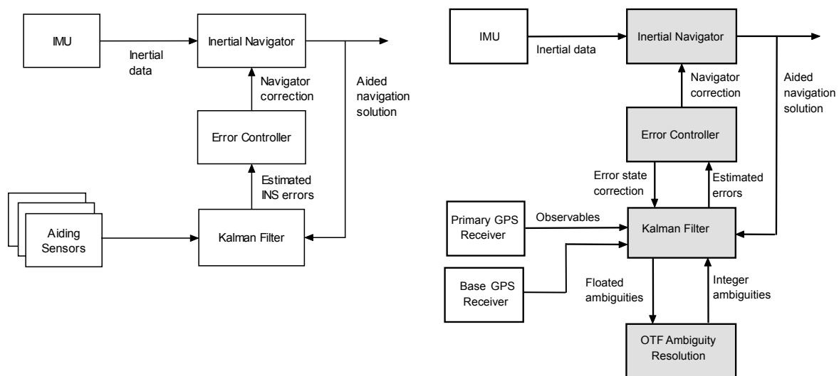
Figure 1: Loosely Coupled Aided Inertial Architecture (left), Tightly Coupled GNSS-Aided Inertial Architecture (right)
