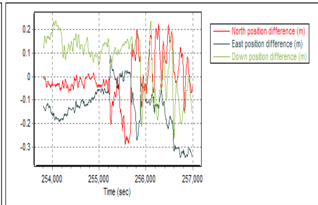
Figure 21: Diff with Reference, PP V4.4, Full Outages
