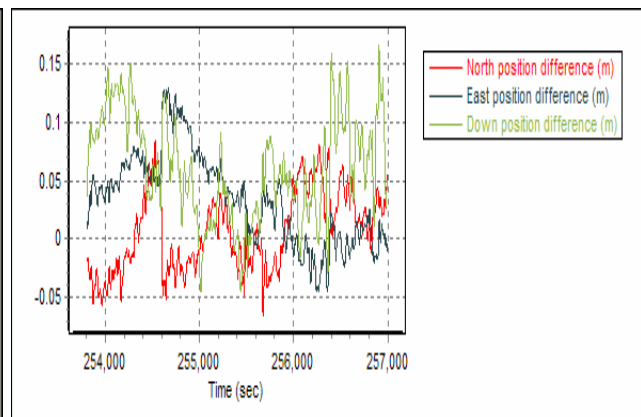
Figure 9: Differences with Reference, PP V5
