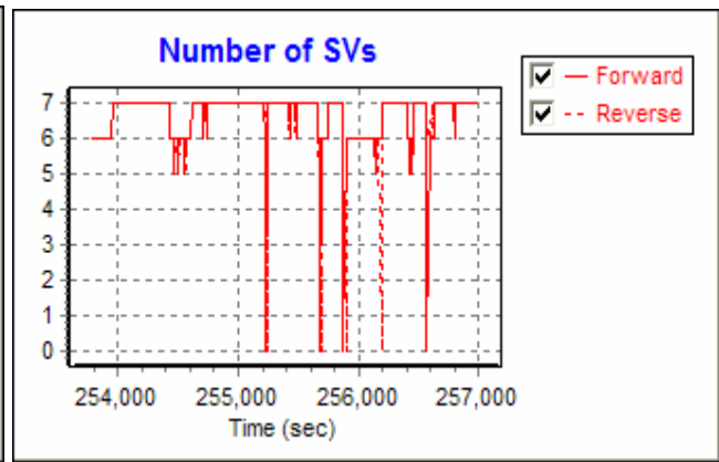
Figure 15: Number of SV's, Full Outages
