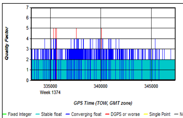
Figure 33: Processing Mode PP V4.4, Sharp Turns Flt2
