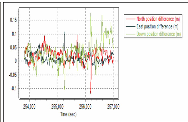
Figure 17: Differences with Reference, Partial Outages
