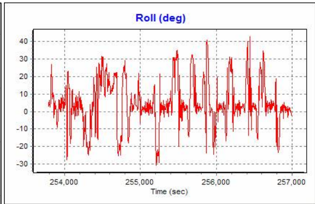
Figure 3: Aircraft Roll
