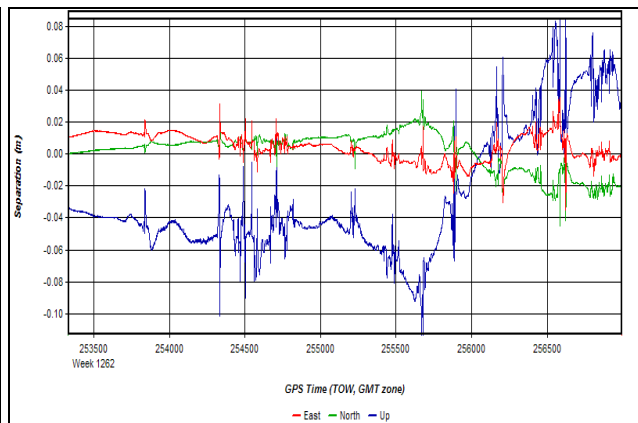
Figure 5: Forward-Reverse Separation, Dedicated Base
