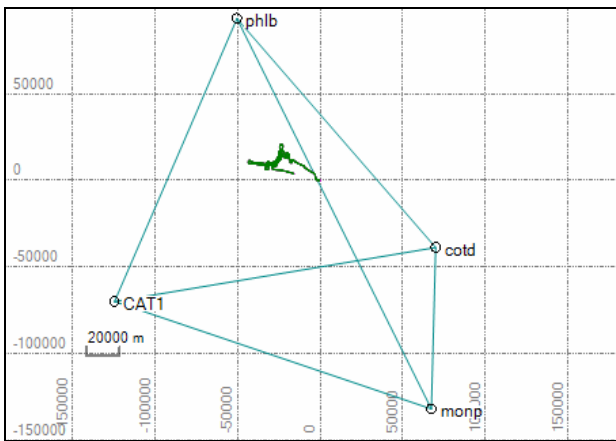
Figure 6: Reference Station Configuration
