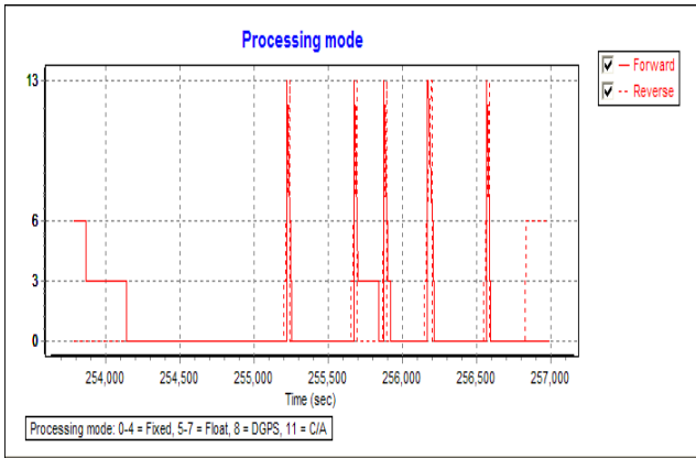
Figure 18: Processing Mode PP V5, Full Outages
