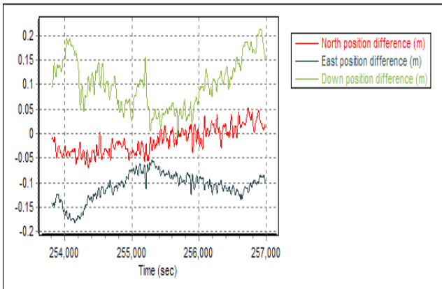
Figure 20: Diff with Reference PP V4.4, Partial Outages
