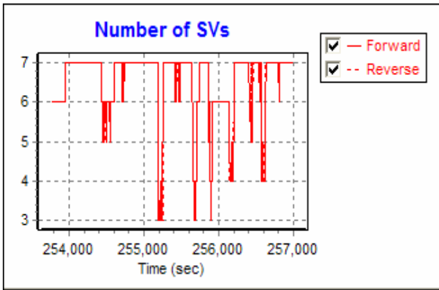
Figure 14: Number SV's, Partial Outages
