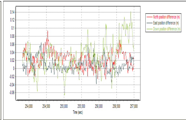
Figure 19: Diff with Reference, PP V5, Full Outages
