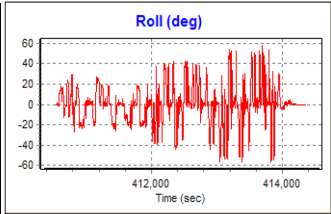
Figure 23: Aircraft Roll, Sharp Turns Flt1
