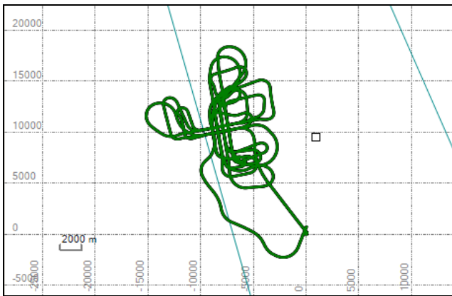
Figure 22: Trajectory, Sharp Turns Flt1
