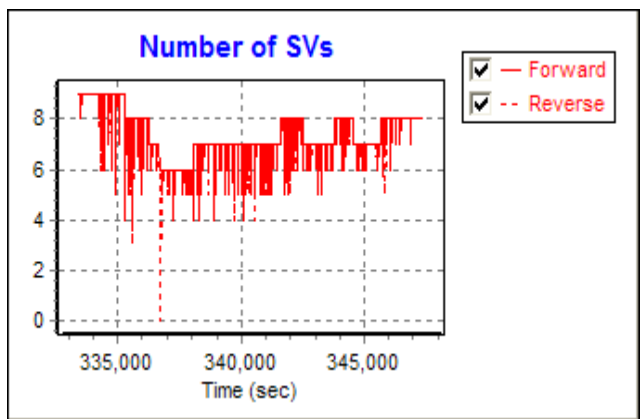
Figure 31: Number of Satellites Tracked
