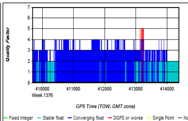
Figure 27: Processing Mode PP V4.4, Sharp Turns Flt1
