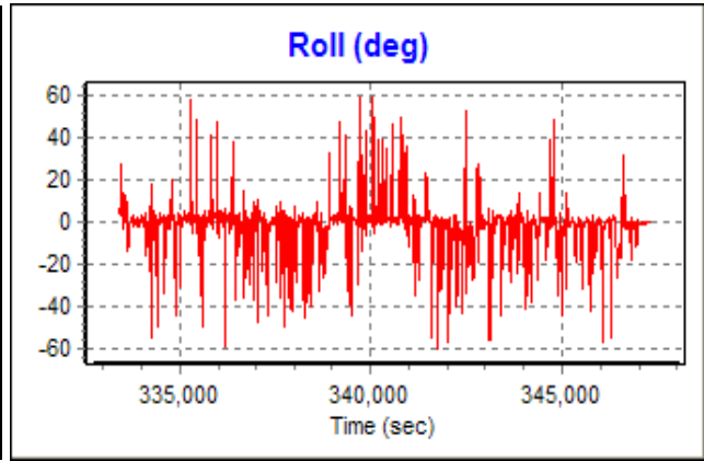
Figure 29: Aircraft Roll, Sharp Turns Flt2
