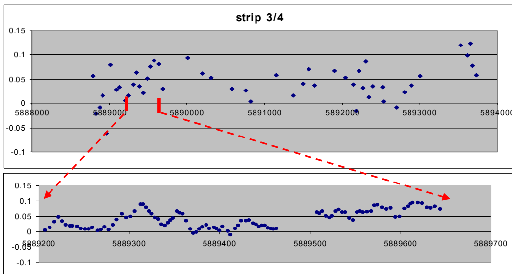
Figure 2: Height discrepancies between neighboring strips in [m]: Top: section of 5km (top), zoomed section of 450m (bottom)
