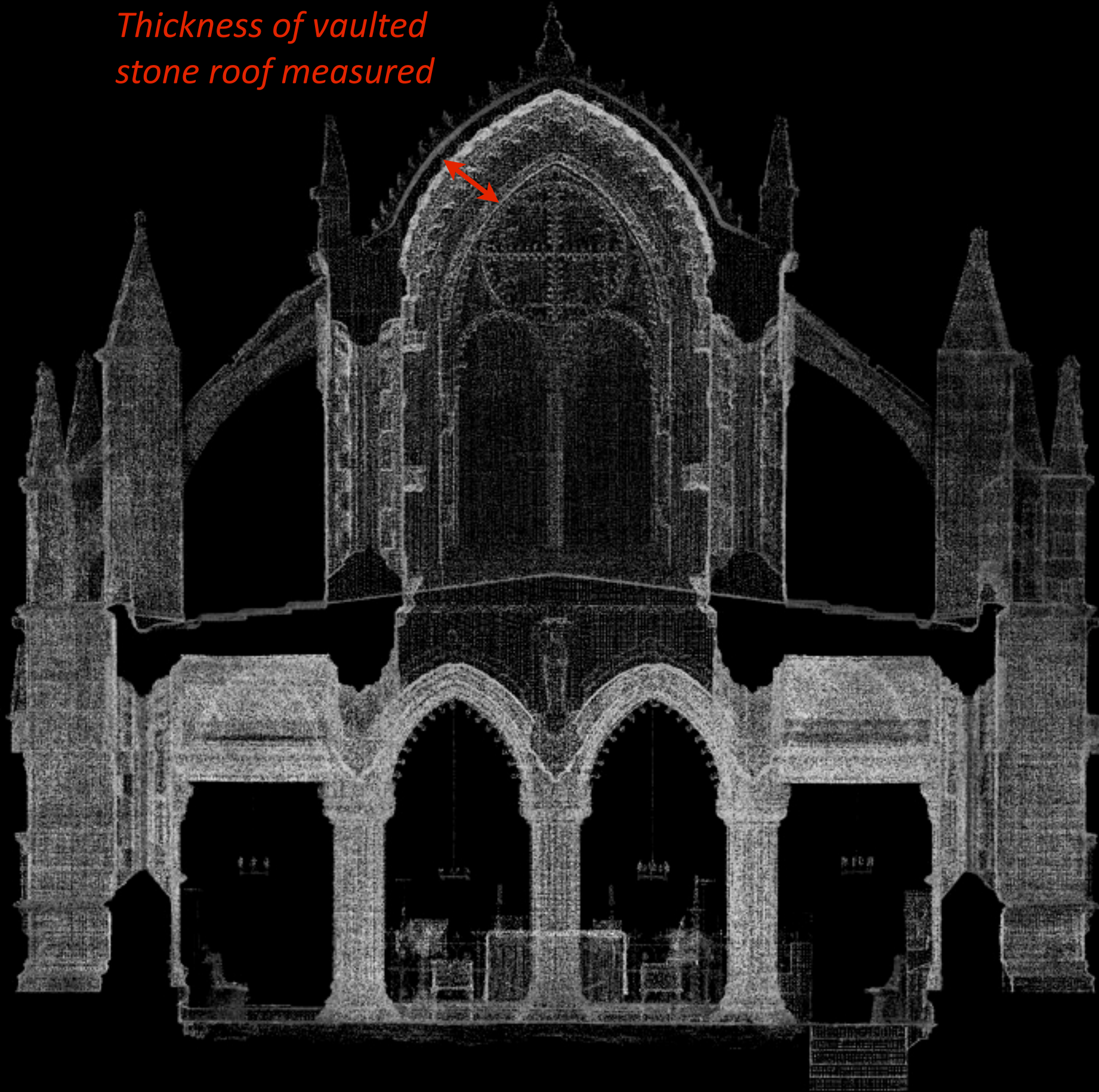
Rosslyn Chapel | Edited point data – cross sections
