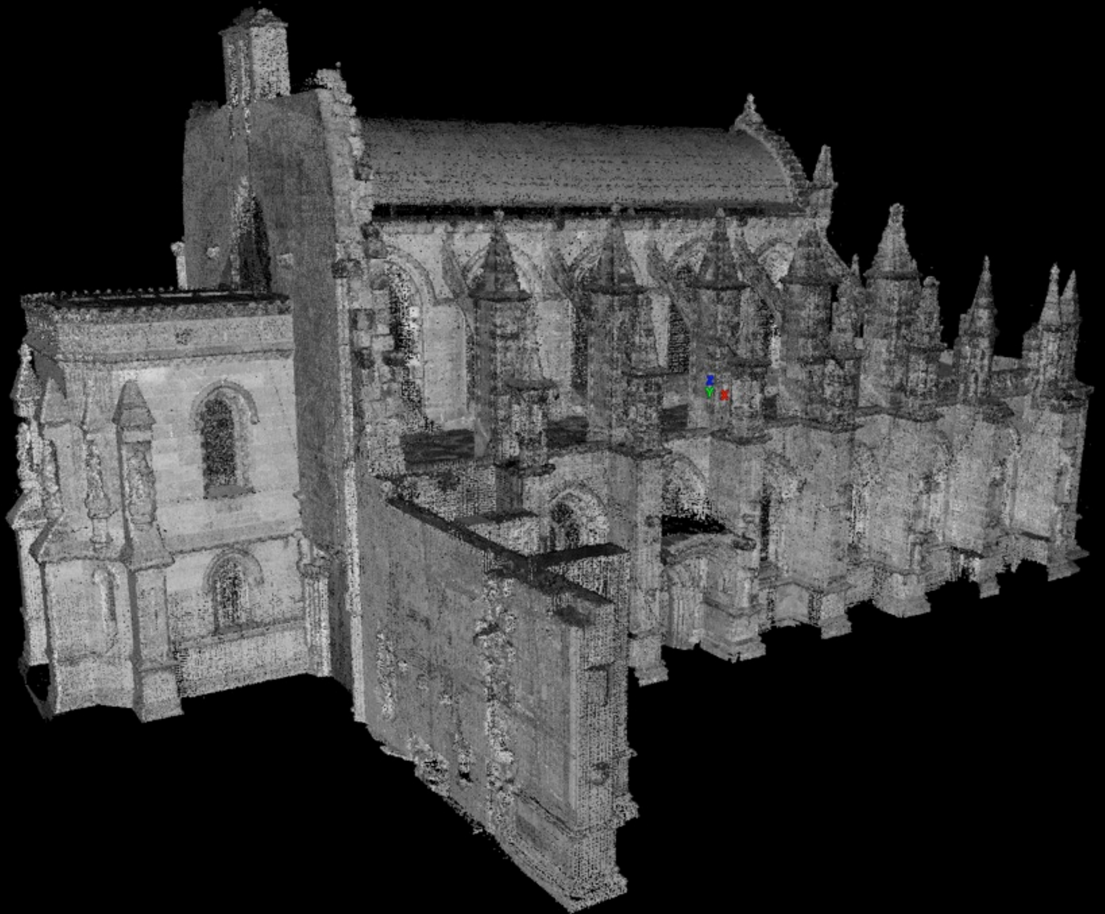
Rosslyn Chapel | Edited point data with the temporary roof and terrain removed
