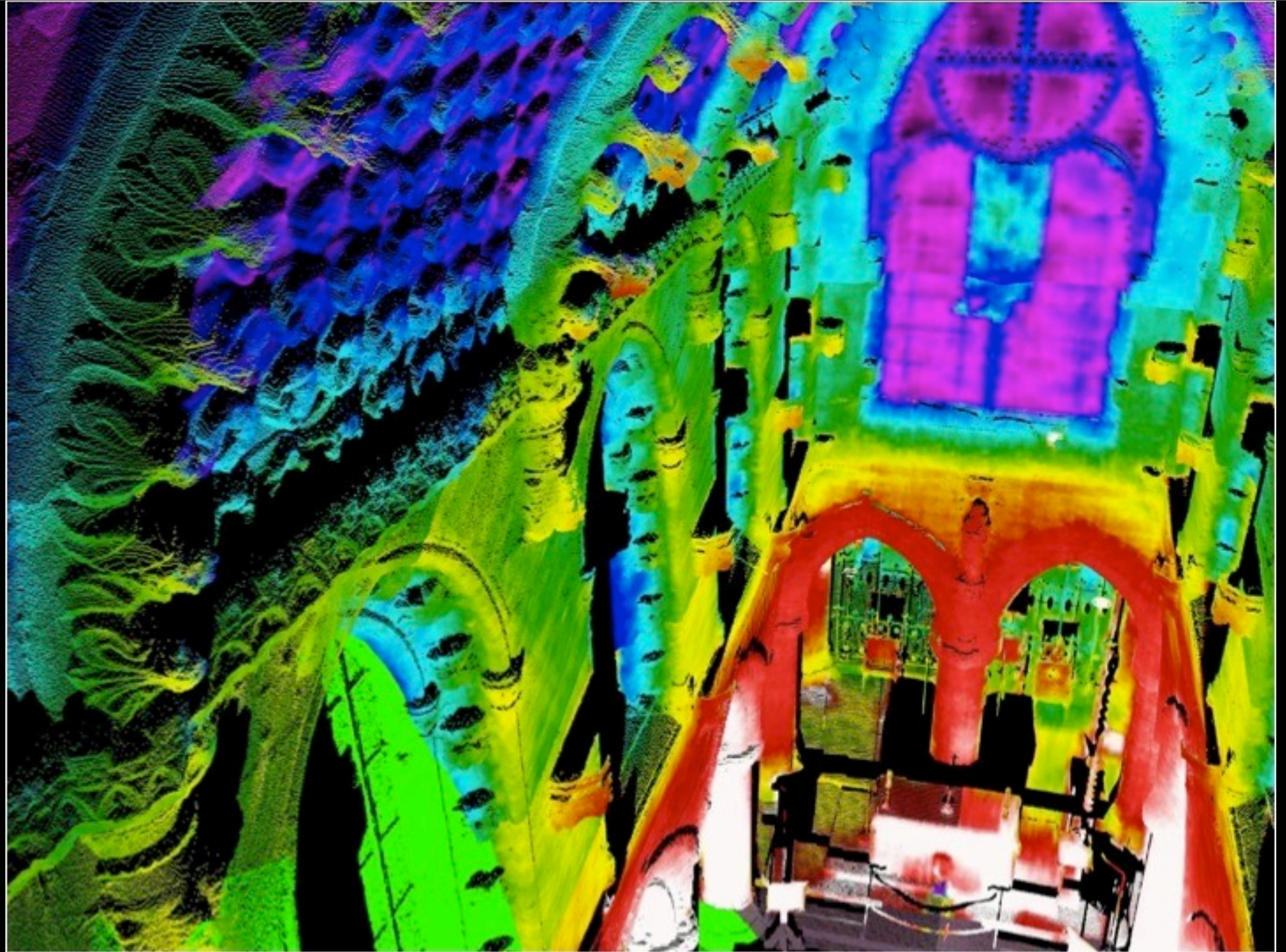
Rosslyn Chapel | Thermal imagery applied to point cloud
